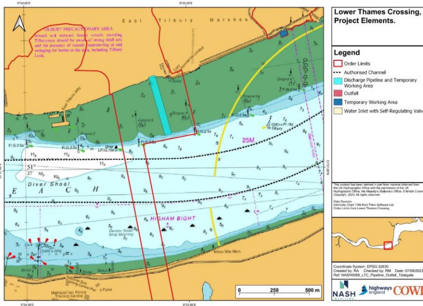
Plate 1.3 Discharge Pipeline, Outfall, Water Inlet with self-regulating valve, Pipeline and Temporary Working Area Locations
