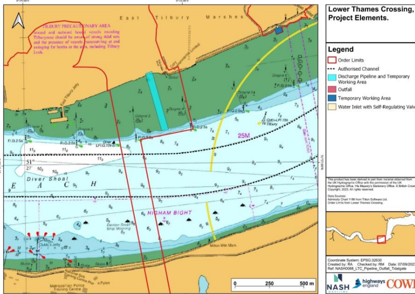
Plate 3.2 Discharge pipeline and outfall locations
