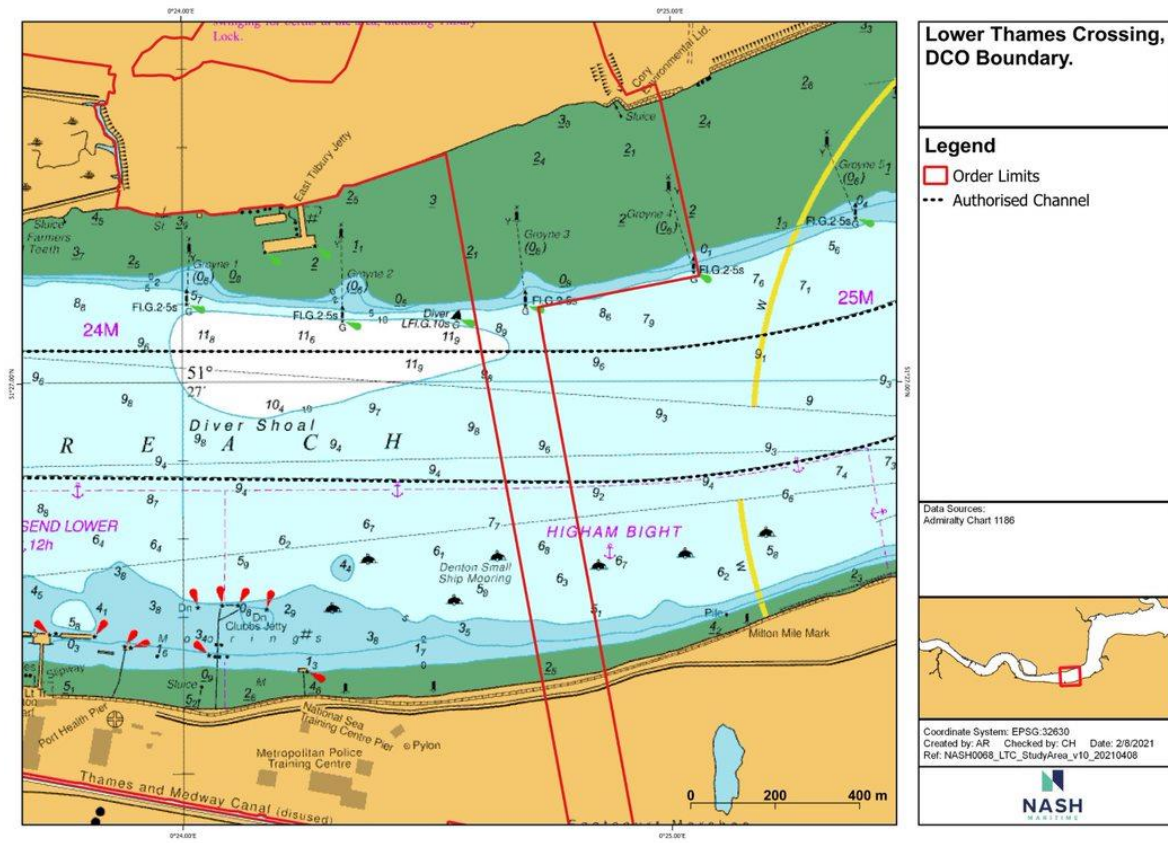
Figure 3: Project Marine Draft DCO Order Limits
