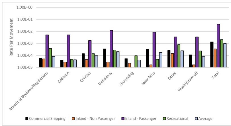
Plate 4.11 PLA recorded incidents 2010–2020 – frequency per vessel movement
